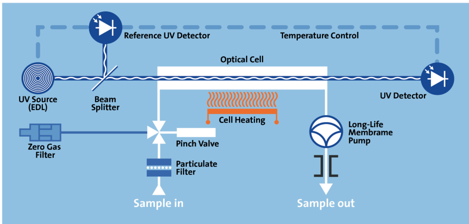
VM-3000 flow chart
